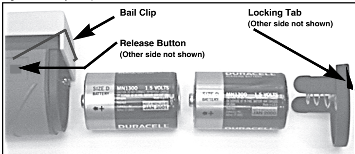
Figure 1. Battery Compartment
